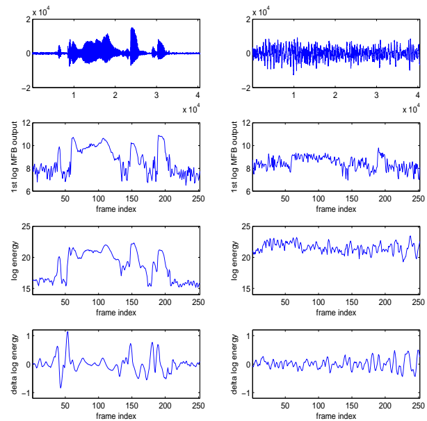
Figure 1: Effect of car noise on log mel-filter bank (MFB) and log energy trajectories. The left subfigures (up to down): waveform, the first log MFB output, log energy, and the delta log energy of close-talking speech; The right subfigures (up to down): waveform, the first log MFB output, log energy, and the delta log energy of distant speech; The speech is “12439” in Japanese.
