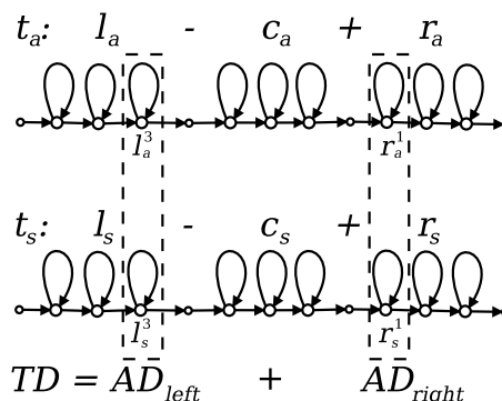
Figure 1: Acoustic triphone distance TD(t_a, t_s) calculation based on acoustic left and right contextual distances, keeping the same center phonemes c_a = c_s .
