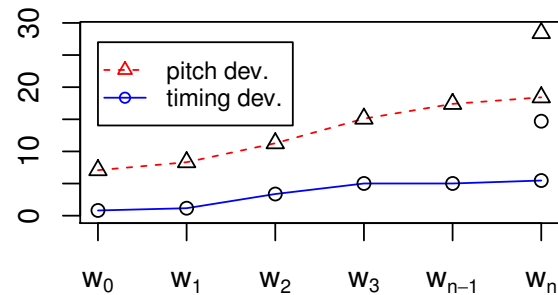
Figure 4: Deviation of pitch and timing plotted against lookahead. The more lookahead available, the better the results. (The single points on the right represent the trivial setting’s performance.)
