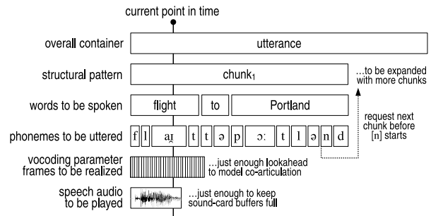
Figure 1: Hierarchic structure of incremental units describing an example utterance as it is being produced during delivery, showing the event-based just-in-time processing strategy.
