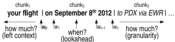
Figure 2: Design space for incremental prosody production. To append the chunk “to PDX via EWR”, we need to decide (a) when to do this, (b) how much left context to use, and (c) how much to add at a time.
