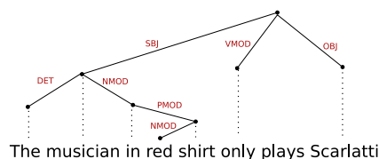
Figure 2: Dependency tree of the sentence "The musician in red shirt only plays Scarlatti"
