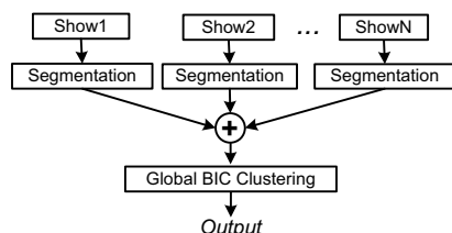
Figure 2: Global-BIC-Seg Cross-show Diarization System
