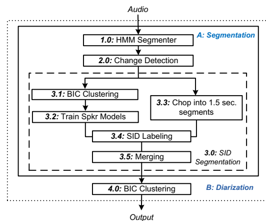
Figure 1: Architecture of the Single-show Diarization System
