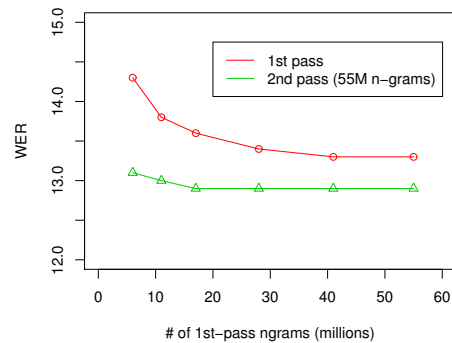
Figure 1: Word error rate with Bayesian interpolation in the first pass with various-sized LMs and dynamic interpolation in the second pass with 55 million n -gram LMs.
