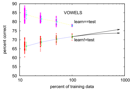
Figure 2: Effect of training data size on classification accuracy. Arrows point to the estimated range of accuracy at 8 times the amount of training data.
