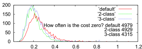
Figure 5: Effect of the target cost on the join cost distribution. The number of joins with a cost of 0 is not plotted on the graph but instead given in the key.
