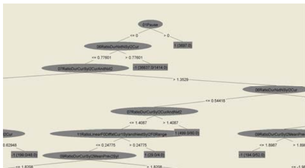
Figure 2: An example of a decision tree for all 16 speakers.
