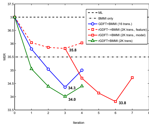
Figure 1: WER of different training procedures using rGDFT on dev set (TransTac Jun08 open set).
