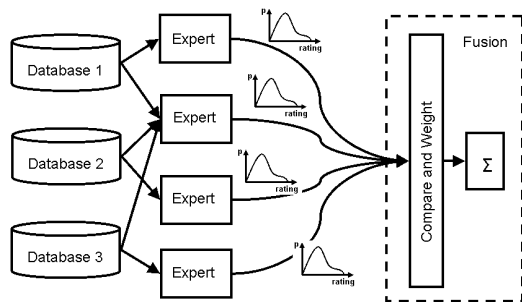
Figure 1. Mixture of Experts as applied in this work.
