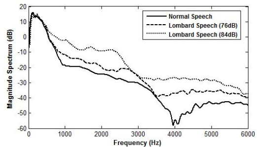
Figure 2: Averaged spectrum for a male speaker uttering in a silent environment, or with a factory noise of 76 dB and 84 dB.
