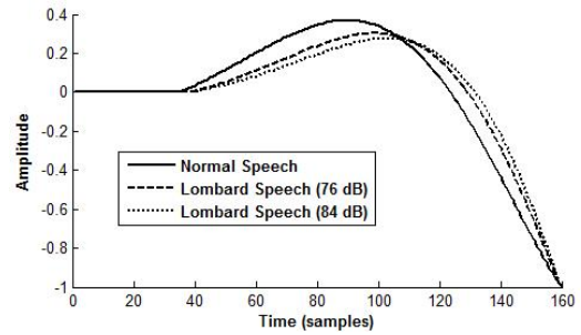
Figure 5: Illustration of the differences in the glottal open phase according to the LF model for normal and Lombard speech.
