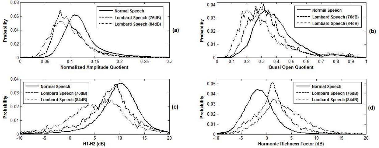
Figure 4: Distributions, for a given male speaker uttering in a quiet environment or in noisy conditions (with a factory noise at 76 and 84 dB), of the following glottal features: (a): the Normalized Amplitude Quotient NAQ , (b): the Quasi-Open Quotient QOQ , (c): the ratio of the amplitudes at the two first harmonics H1-H2 , (d): the Harmonic Richness Factor HRF .
