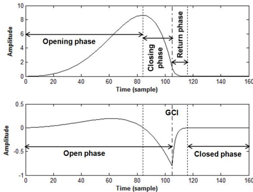
Figure 1: Typical waveforms, according to the Liljencrants-Fant (LF) model, of one cycle of: (top) the glottal flow, (bottom) the glottal flow derivative. The various phases of the glottal cycle, as well as the Glottal Closure Instant (GCI) are also indicated.
