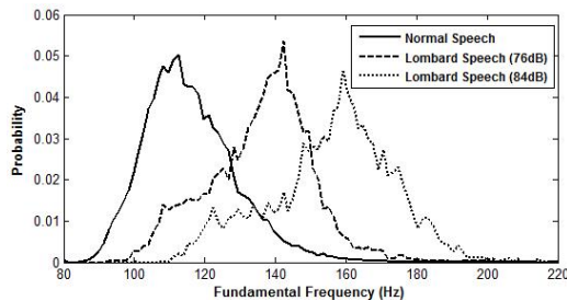
Figure 3: Pitch distribution for a given male speaker uttering in clean and noisy conditions. For this example, a factory noise at 76 and 84 dB was used.
