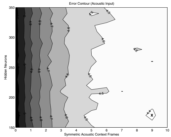
Figure 4: Contour plot of EPG estimation error versus number of symmetric frames and number of hidden neurons when only acoustic parameters are used at the networks’ input. X marks the minimum.
