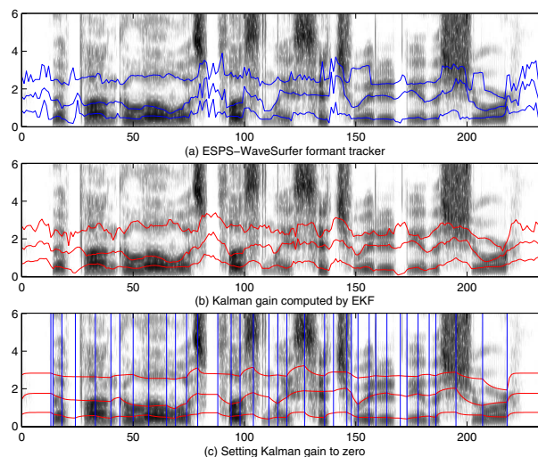
Figure 1: Spectrogram of a TIMIT utterance superimposed with (a) formant tracker data, and recovered VTR sequences from the full HDM (b) and from the “partial” HDM using only the predictor step of the EKF recursion (c).
