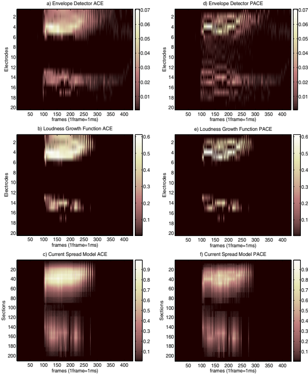
Figure 5: a) Acoustic Envelope with ACE, b) Loudness Growth Function with ACE, c) Current spread with ACE, d) Acoustic Envelope with PACE, e) Loudness Growth Function with PACE, f) Current Spread with PACE.
