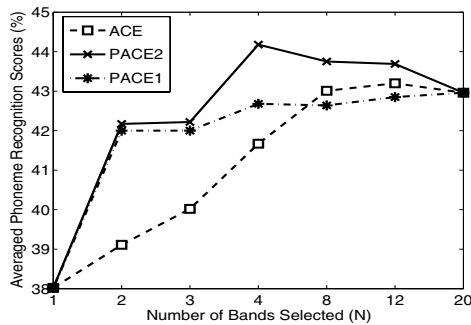
Figure 7: Phoneme Recognition Results.
