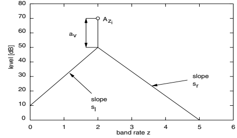
Figure 4: Spreading Function.
