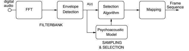
Figure 3: PACE strategy block diagram.
