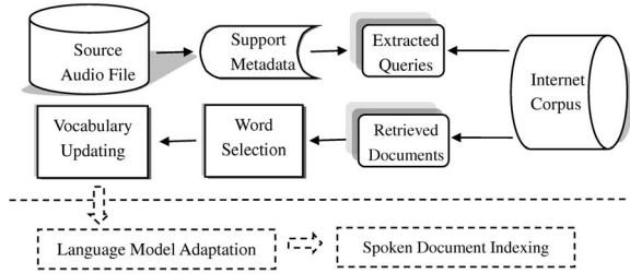
Figure 1: A system for single-document online vocabulary and language model adaptation
