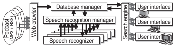
Figure 3: Implementation overview of PodCastle.
