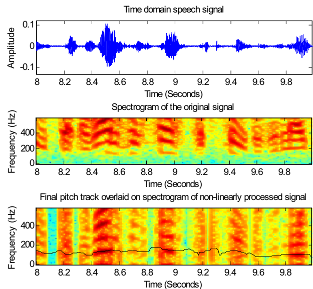
Figure 6. Illustration of the spectral pitch tracking
