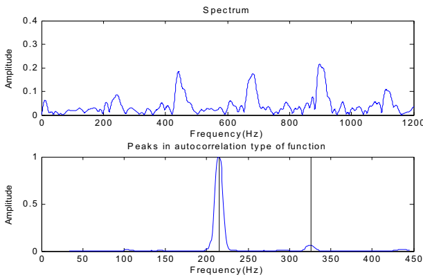
Figure 4. Peaks in autocorrelation type of function
