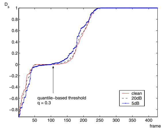
Figure 2: Quantile-based adaptive threshold for different SNRs.
