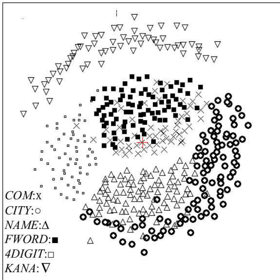
Figure 1 Multi Task COSMOS Map
