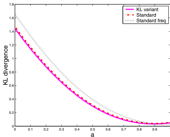
Figure 3: KL divergence to q_i(a) distribution.
