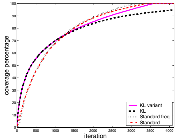
Figure 2: Evolution of triphone coverage.
