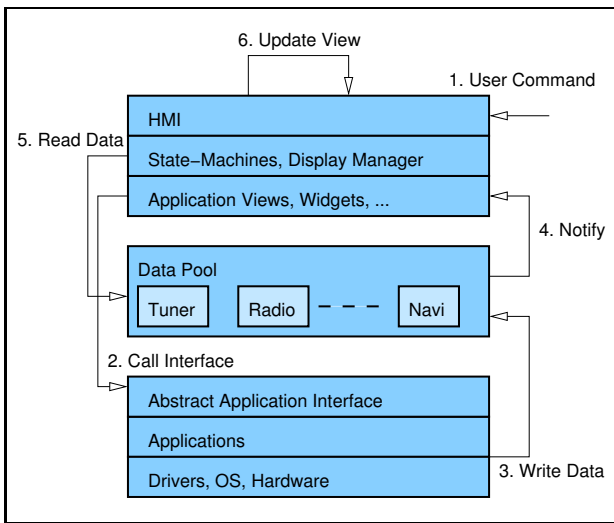
Figure 1: Data Pool Architecture of tresos GUIDE
