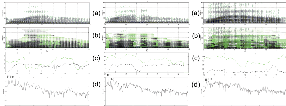
Fig 1 : Spectrogram (a) & Spectro-Temporal Profile (b) for a Modal (Left), Breathy (Middle) and Creaky voice (Right); green dots represent aperiodicity and black dots represent periodicity content. The figures (c) show the summary aperiodicity (green) and periodicity (black) measure, while (d) show a spectrum slice for each case
