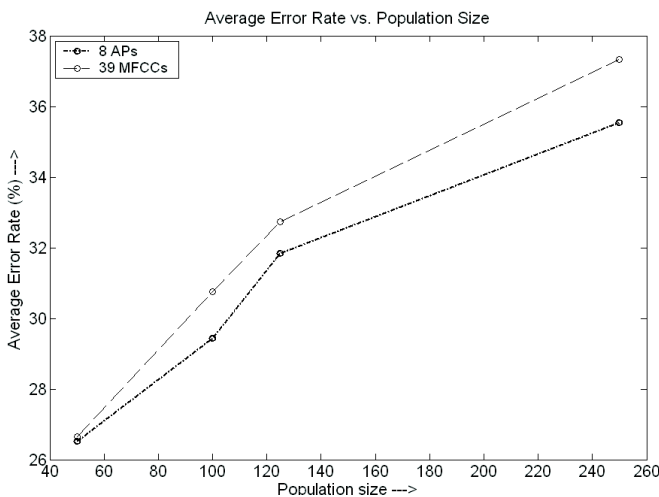
Figure 4: Average Error Rate vs. Population Size
