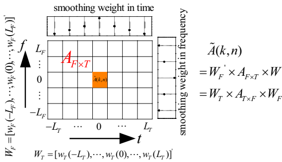
Figure 1: Spectrum smoothing in time and frequency index
