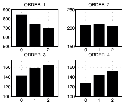
Figure 1: Perplexities of the foreground reference words during nonoverlaps (0), single-speaker overlaps (1), and two-speaker overlaps (2), for various n -gram LMs.
