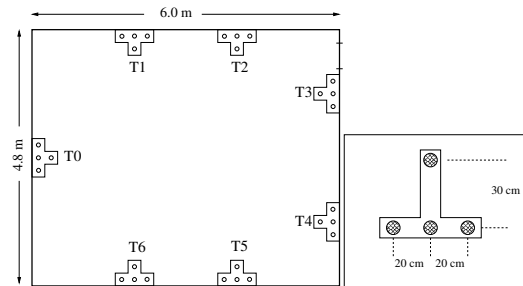
Figure 1: The CHIL room available at ITC-irst and the geometry of a T-shaped microphone array.
