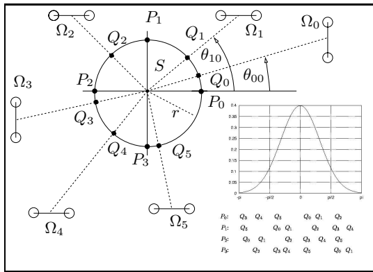
Figure 3: Graphical representation of the orientation estimation scheme described in Sec.4. In this case 6 microphone pairs are available and 4 possible orientations are investigated.
