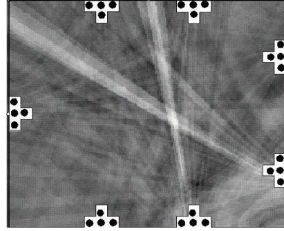
Figure 2: CSP-based 2-dimensional GCF computed in the CHIL room available at ITC-irst. GCF magnitude is represented by gray levels. The brightest spot corresponds to the speaker position.
