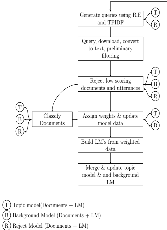
Fig. 1. System overview. For the first iteration the system has a dummy reject model.
