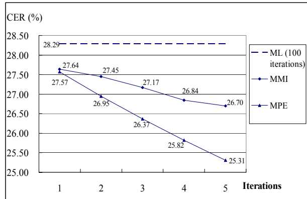
Figure 2: The speech recognition results (CERs) for three different baseline systems trained with ML, MMI and MPE criteria, respectively.
