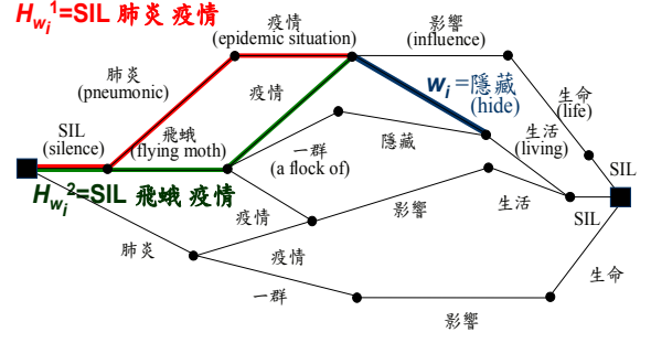
Figure 1: An illustration of the word graph, in which each arc, together with its corresponding start and end speech frames, represents a candidate word hypothesis.
