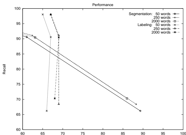
Figure 4: Varying the POS model: The performance of the models slowly improves as long as only a small number of words are mapped onto their parts of speech. The improvements level off fairly quickly but without any over-training effects. See also Figure 3.
