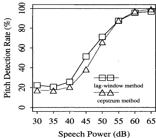
Figure 2: Performance comparison between the lag-window method and the cepstrum method
