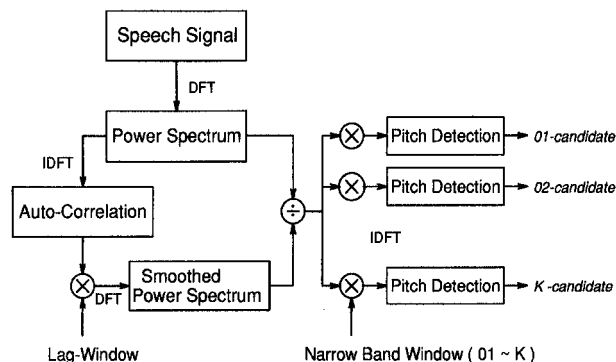
Figure 3: Block diagram of pitch extraction by narrow band spectrum analysis
