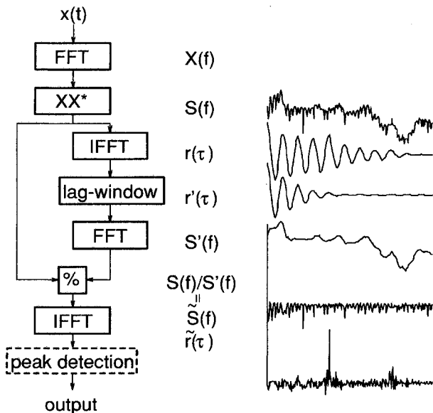
Figure 1: Block diagram of a basic pitch analysis with lag-window method
