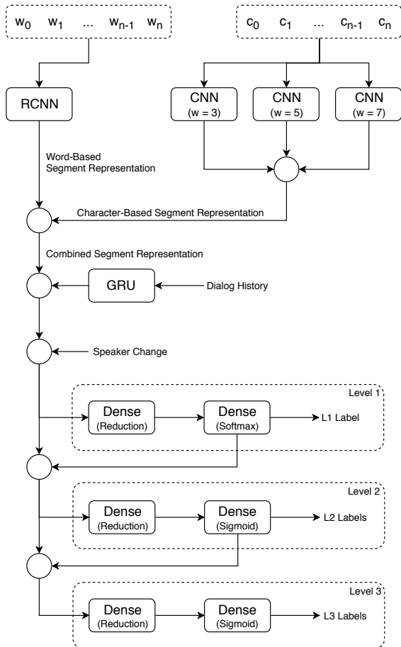
Figure 1: The architecture of our network. w_i refers to the embedding representation of the i -th word, while c_i refers to the embedding representation of the i -th character. The circles represent the concatenation of the different inputs.
