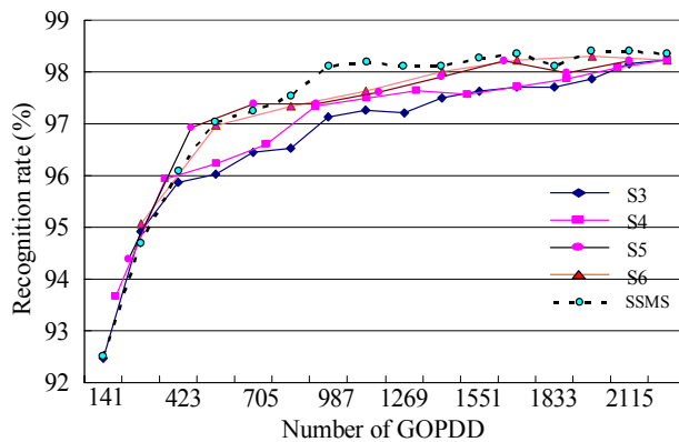
Figure 6. Comparison of recognition rate of SI fixed parameter model and SI variable parameter model using SSMS. (# GOPDD = # phone: 47 × # state: 3~6 × # mixture: 1~16)
