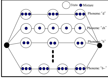
Figure 1. An example of variable parameter model topology
