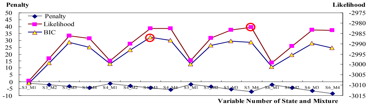
Figure 2. Log likelihood, penalty, and BIC of Korean phoneme "aa"
