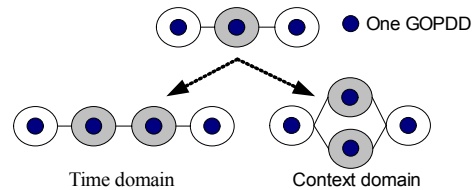
Figure 5. An example of splitting in time and context domains
