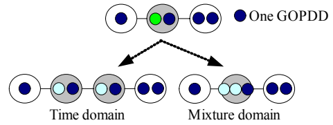
Figure 4. An example of splitting in time and mixture domains
