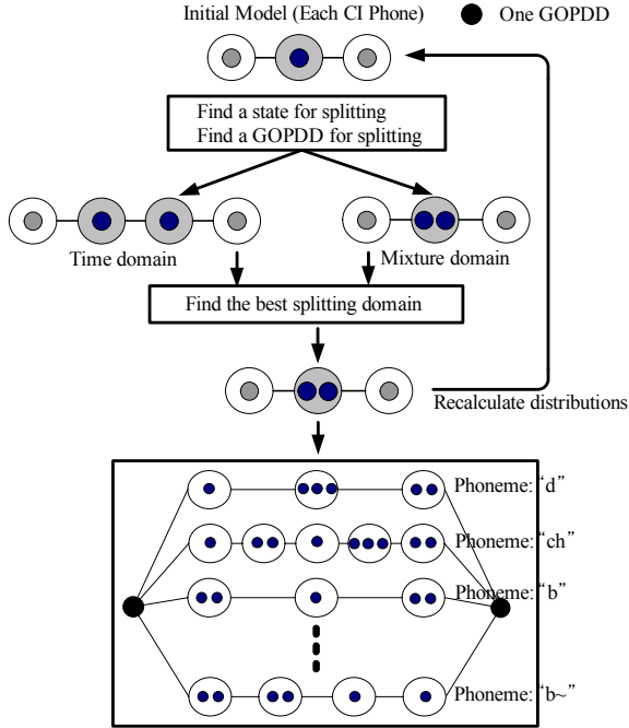
Figure 3. Generation of SSMS model
