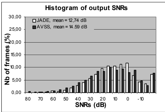
Figure 1 : 2 sensors, 2 sources - Matrix A1 - T=1
