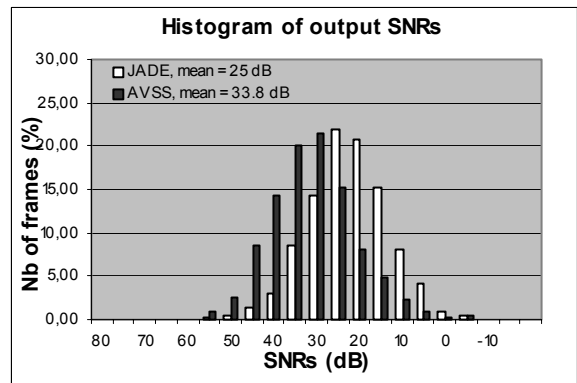
Figure 5 : 3 sensors, 3 sources - Matrix A1 - T=20
