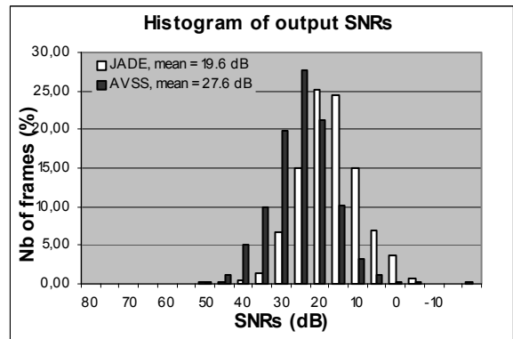
Figure 6 : 5 sensors, 5 sources - Matrix A1 - T=20
