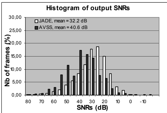
Figure 3 : 2 sensors, 2 sources - Matrix A1 - T=20
