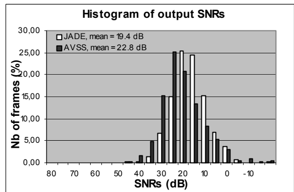
Figure 7 : 5 sensors, 5 sources - Matrix A2 - T=20
