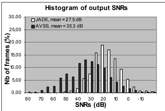
Figure 2 : 2 sensors, 2 sources - Matrix A1 - T=10
