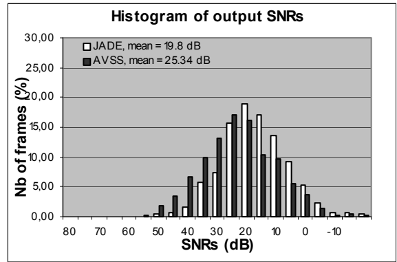
Figure 4 : 3 sensors, 3 sources - Matrix A1 - T=10
