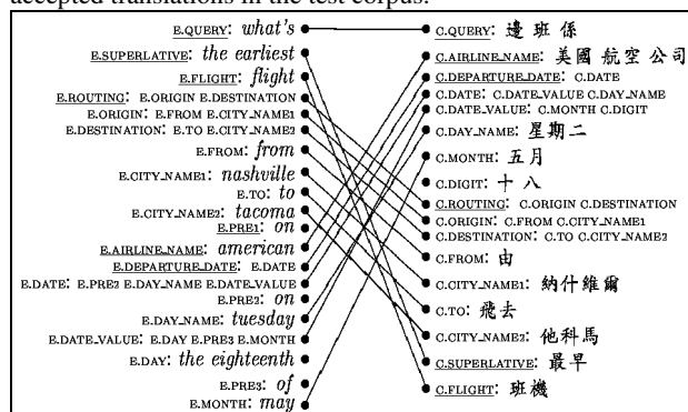
Figure 2: Example template with aligned English-Chinese concept-value pairs. Top level concepts are underlined.
