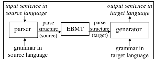
Figure 1: Overview of our bi-directional machine translation framework that uses semi-automatically induced parallel grammars.
