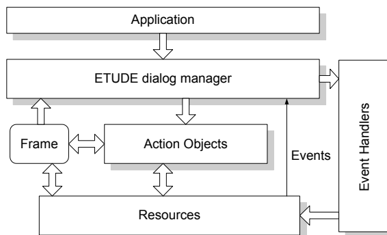
Figure 3: Multi-modal architecture.
