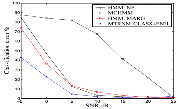
Figure 3: RNN performance on classification
