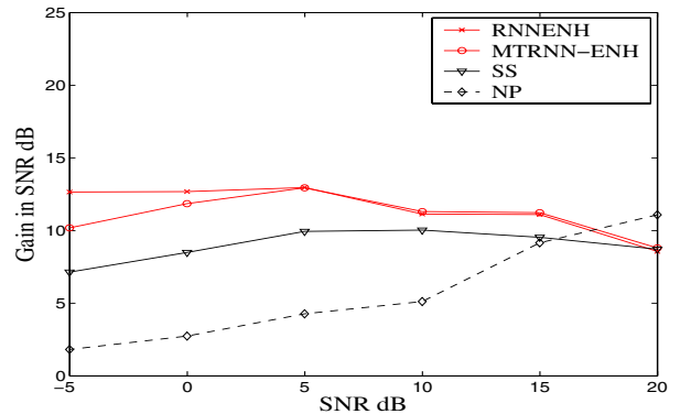
Figure 4: RNN performance on pattern completion
