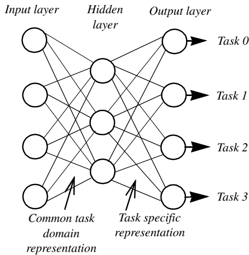
Figure 1: An MTL network with one main task and three extra tasks. There is an output unit for each task being learned in parallel
