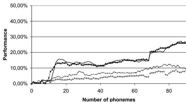
Figure 7: Speaker identification performance when the training data came from the desk microphone and the test data came from the close-talking microphone. Dashed line = identification based on the likelihood of the whole utterance; line of crosses = identification based on the majority voting rule for single phonemes; solid line = identification based on the majority voting rule for sequences of 10 phonemes; line of triangles = identification based on the majority voting rule for sequences of 7 phonemes.
