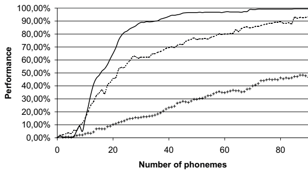
Figure 5: Speaker identification performance when both the training and test data came from the desk microphone. Dashed line = identification based on the likelihood of the whole utterance; line of crosses = identification based on the majority voting rule for single phonemes; solid line = identification based on the majority voting rule for sequences of 8 phonemes.
