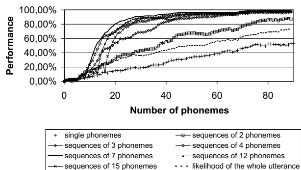
Figure 4: Determination of the optimal number of phonemes for the procedure based on the majority voting rule for sequences of phonemes.
