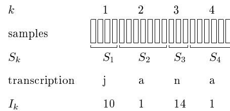
Figure 1: An illustration of assigning indexes I_k to segments S_k .
