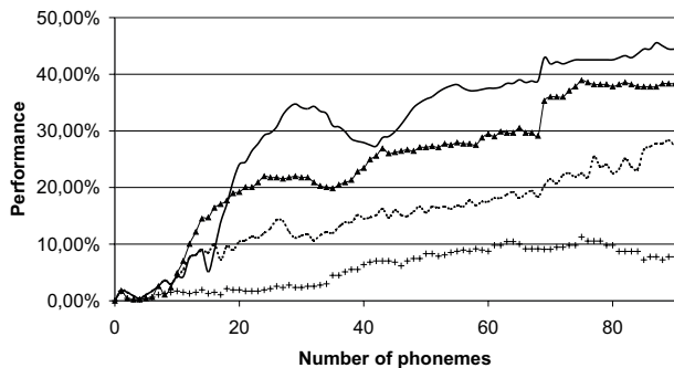
Figure 6: Speaker identification performance when the training data came from the close-talking microphone and the test data from the desk microphone. Dashed line = identification based on the likelihood of the whole utterance; line of crosses = identification based on the majority voting rule for single phonemes; solid line = identification based on the majority voting rule for sequences of 14 phonemes; line of triangles = identification based on the majority voting rule for sequences of 7 phonemes.
