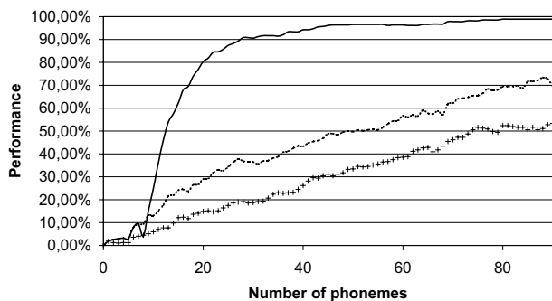
Figure 3: Speaker identification performance when both the training and test data were obtained from the close-talking microphone. Dashed line = identification based on the likelihood of the whole utterance; line of crosses = identification based on the majority voting rule for single phonemes; solid line = identification based on the majority voting rule for sequences of 7 phonemes.
