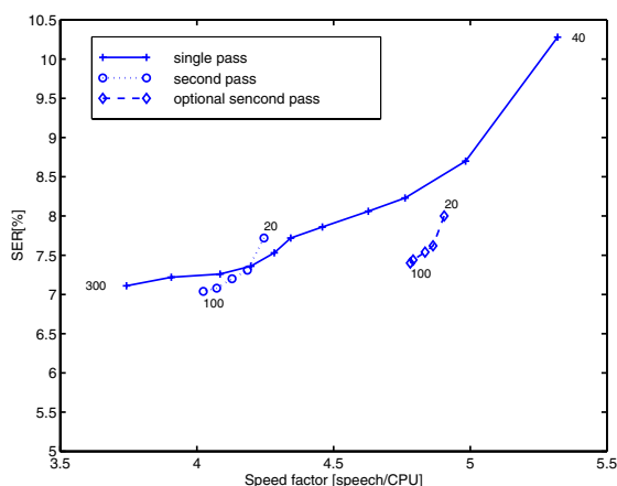
Figure 1: Speed/error rate dependency on the stock name task
