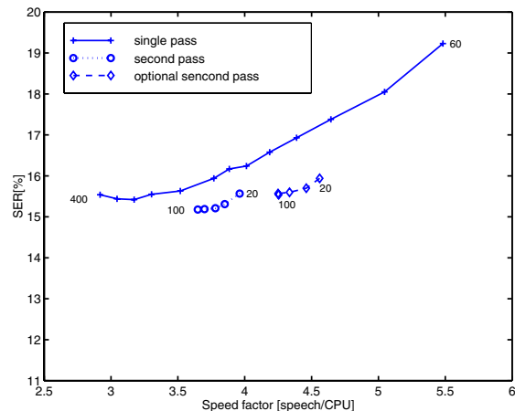
Figure 2: Speed/error rate dependency on the name dialer task
