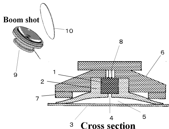
Figure 2. Stethoscopic microphone:
