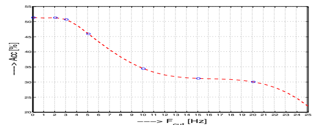
Figure 3: Dependence of phoneme recognition accuracy on F_{cutoff} , when the lower spectral components are discarded.
