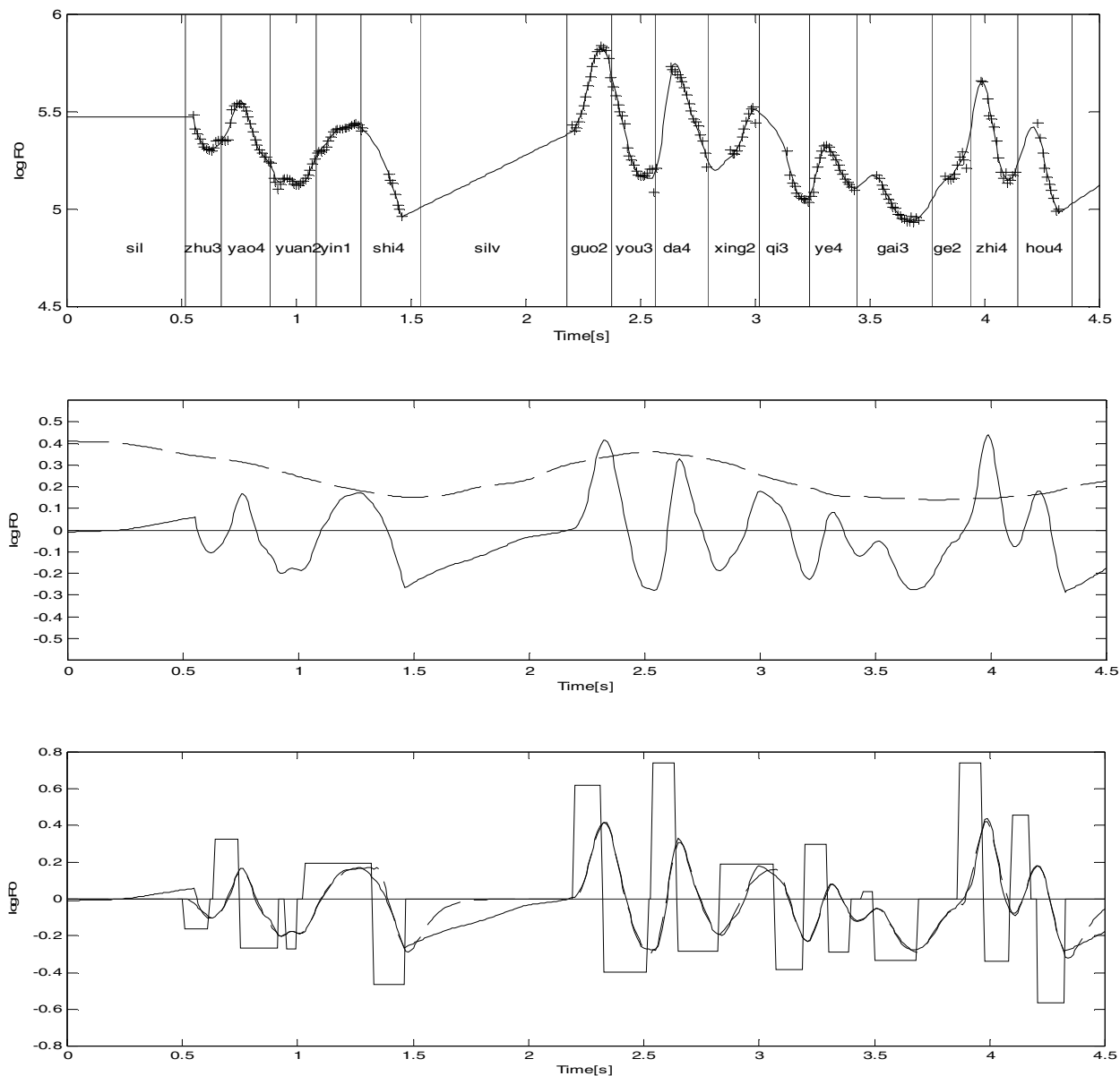
Figure 1. Top: Example of extracted (+ signs) and interpolated/smoothed (solid line) F_0 contours from the corpus. Center: HFC (solid) and LFC (dashed) reduced by F_b . The HFC oscillates around zero, with excursions suggesting underlying positive or negative tone commands. Local minima in the LFC indicate the approximate positions of subsequent phrase commands, except for the first phrase command which is located before the onset of the utterance. Bottom: Tone command sequence and resulting model contour (dashed) as compared with the HFC (solid line) after the first optimization stage.
