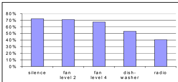
Figure 5: Dependency of the recognition rate on the background noise (recognizer 7, average of all speaker positions)
