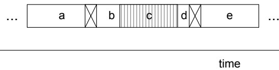
Figure 4: Structure of the audio signal in the positive test: pause wave with background noise I (a), test wave with background noise I (with pause before spoken command (b), spoken command (c), pause after spoken command (d)) and pause wave with background noise II (e).
