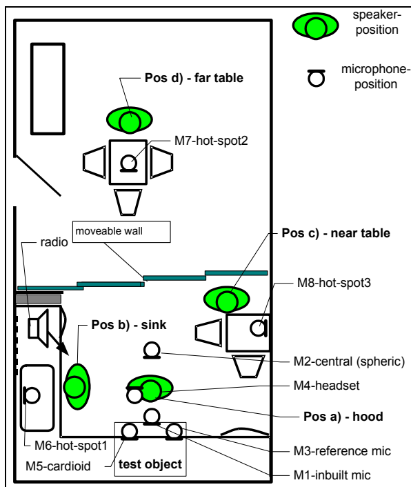
Figure 2: Plan of the usability lab together with microphone and subjects positions.
