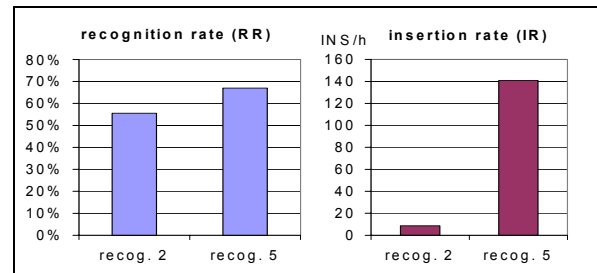
Figure 7: Comparison of two pairs of recognition and insertion rates (recognizer 2 and 5)
