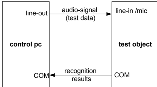
Figure 3: Test configuration
