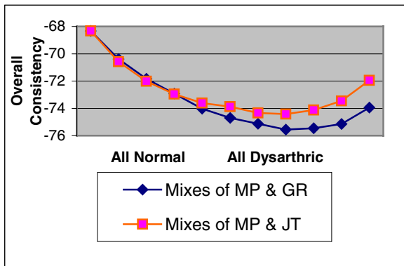
Figure 1: Consistency of Mixed Data Sets
