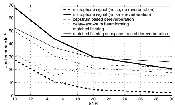
Figure 4: WER vs. SNR for uncorrelated white noise
