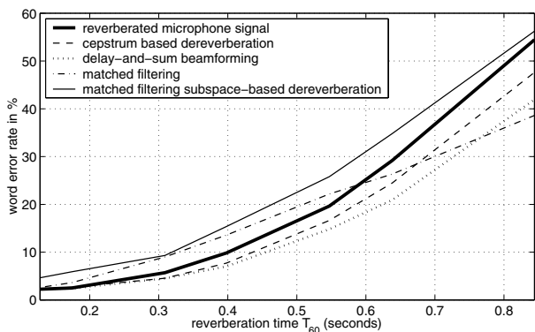
Figure 2: Performance (WER) vs. reverberation time
