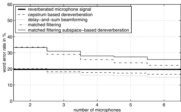
Figure 3: Performance (WER) vs. number of microphones
