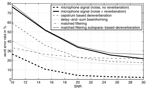
Figure 5: WER vs. SNR for spatially correlated white noise
