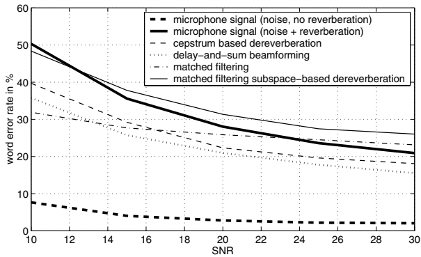
Figure 6: WER vs. SNR for spatially correlated speech-like noise
