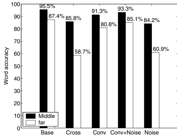
Figure 1: Average results for the middle- and far-talk microphones for the Hebrew SPEECON Database.
