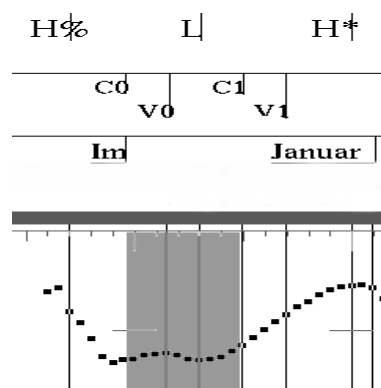
Figure 1: Suprasegmental and segmental labels, together with lexical information (“im JANUAR”, with shaded stress). Lexical labels mark the end of words. Segmental labels mark the start, suprasegmental labels the target point.
