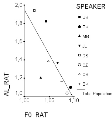
Figure 2: Correlation between the ratio of f_0(H^*) (contrastive:non-contrastive) and the ratio of al(H^*, V1) (contrastive:non-contrastive). One speaker was excluded because she did not realise a difference between the two contrast conditions.
