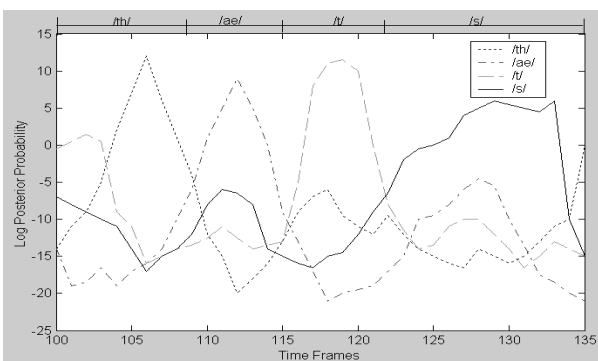
Figure 1. Normalized posterior probability estimates and alignment of the phones in an utterance “That’s”
