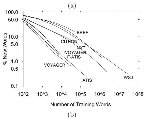
Figure 6: (a) The number of unique words (i.e., task vocabulary) as a function of the size of the training corpora, for several spoken language tasks, and (b) The percentage of unknown words in previously unseen data as a function of the size of the training corpora used to determine the vocabulary empirically. The sources of the data are: F-ATIS=French ATIS; I-VOYAGER=Italian VOYAGER; BREF=French La Monde; NYT=New York Times; WSJ=Wall Street Journal; and CITRON=Directory Assistance.
