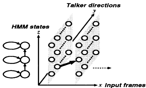
Figure 4. Viterbi search on 3-D trellis space
