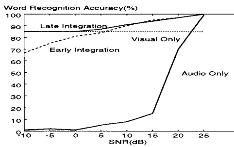
Figure 7. Comparison of Integration Methods
