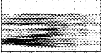
Figure 3. spectrogram of reverberant speech /ai/: T_{60}=600\text{msec}
