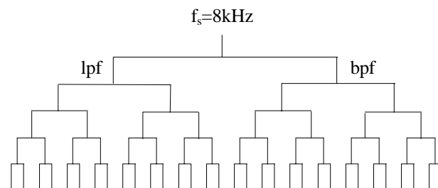
Fig. 1: WPT decomposition structure
