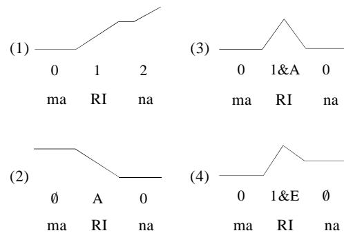
Figure 1. Stylized examples of the four accent-lending shapes on the proper name 'Marina'.
